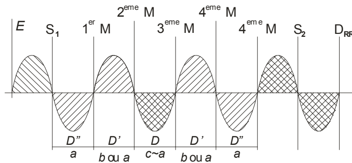
Figure 3. Judgment experience: representation of electromagnetic waves in resonance in the prolonged side of Mach-Zehnder non-equilibrated interferometer when b = n \cdot L / 2 .
