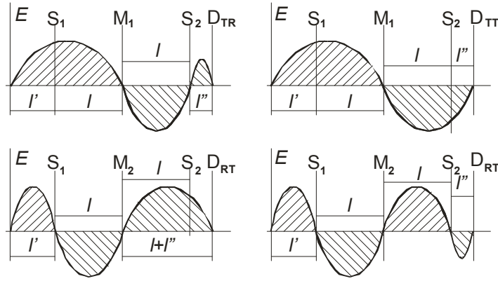
Figure 2. Different possibilities of waves vibration in equilibrated Mach-Zehnder interferometer.
