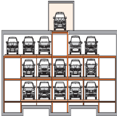
Fig. 1. Automated car parking
