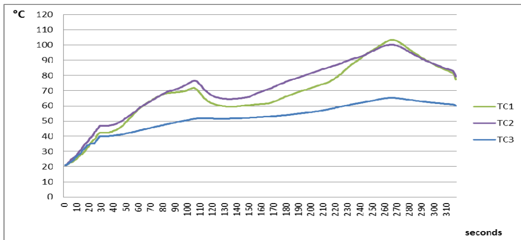
Fig. 2 Temperature evolution inside the fire compartment
