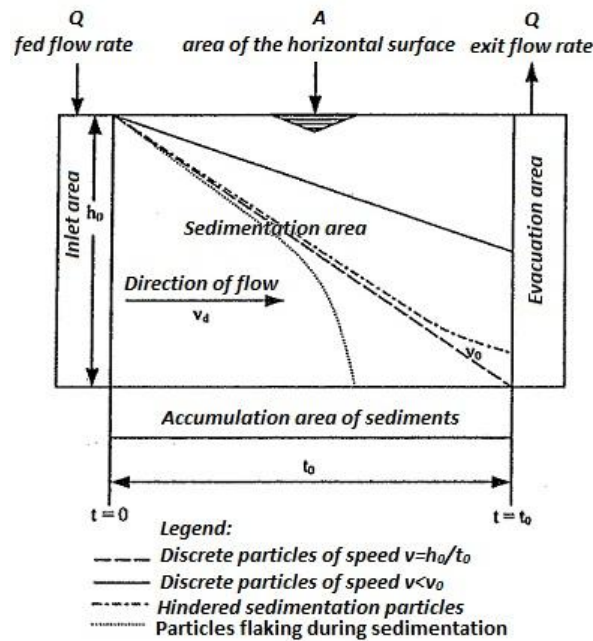
Figure 2. Schematic defining the parameters of a conventional decanter
