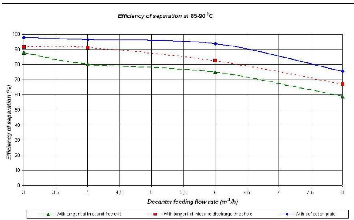
Figure 10. Evolution of the separation efficiency versus flow rate at 85-90°C, for various types of decanters
