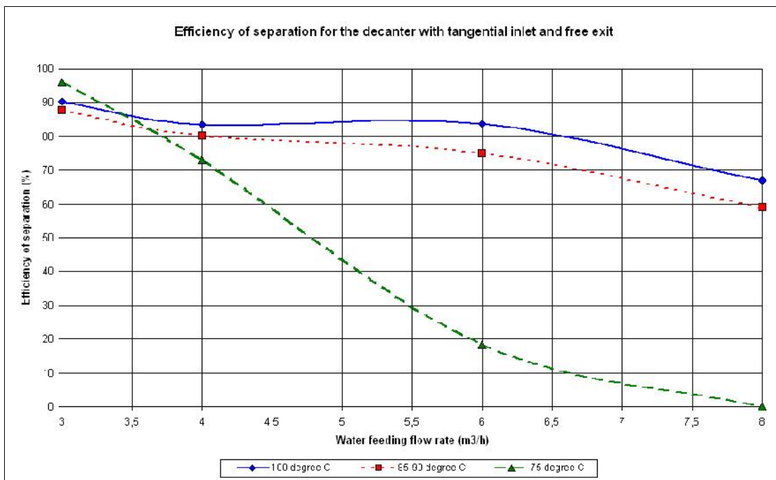
Figure 6. Evolution of the separation efficiency versus feeding flow rate for the decanter D1 with tangential inlet and free exit (see fig. 3) at different wastewater temperatures
